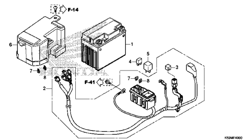
BATTERY
