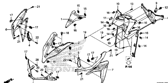
FRONT COVER
