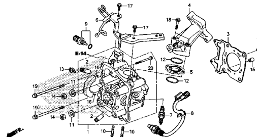
CYLINDER
